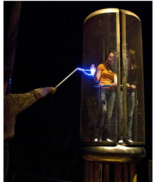
"Cage de Faraday" by Antoine Taveneaux. CC-BY-SA 3.0 http://commons.wikimedia.org/wiki/File:Cage_de_Faraday.jpg
